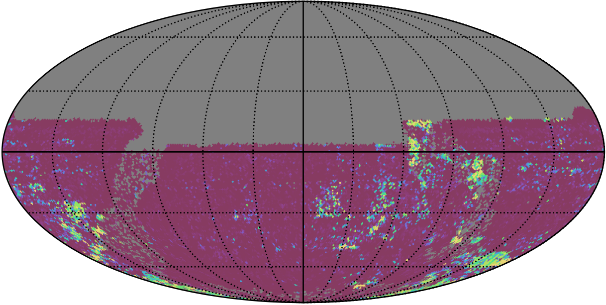
ddf_loaded_half_fl4_v3.4_10yrs All sky u band: 75th Percentile Intranight Timespan
