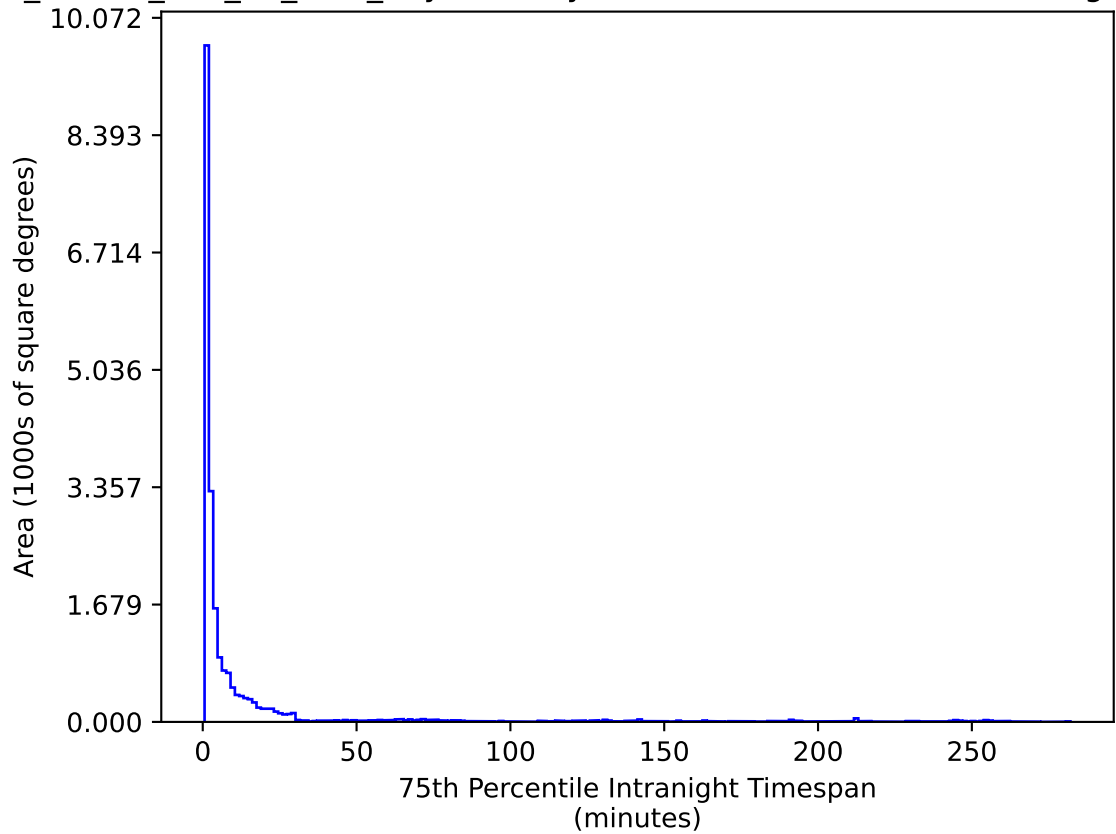
ddf_loaded_half_fl4_v3.4_10yrs All sky u band: 75th Percentile Intranight Timespan
