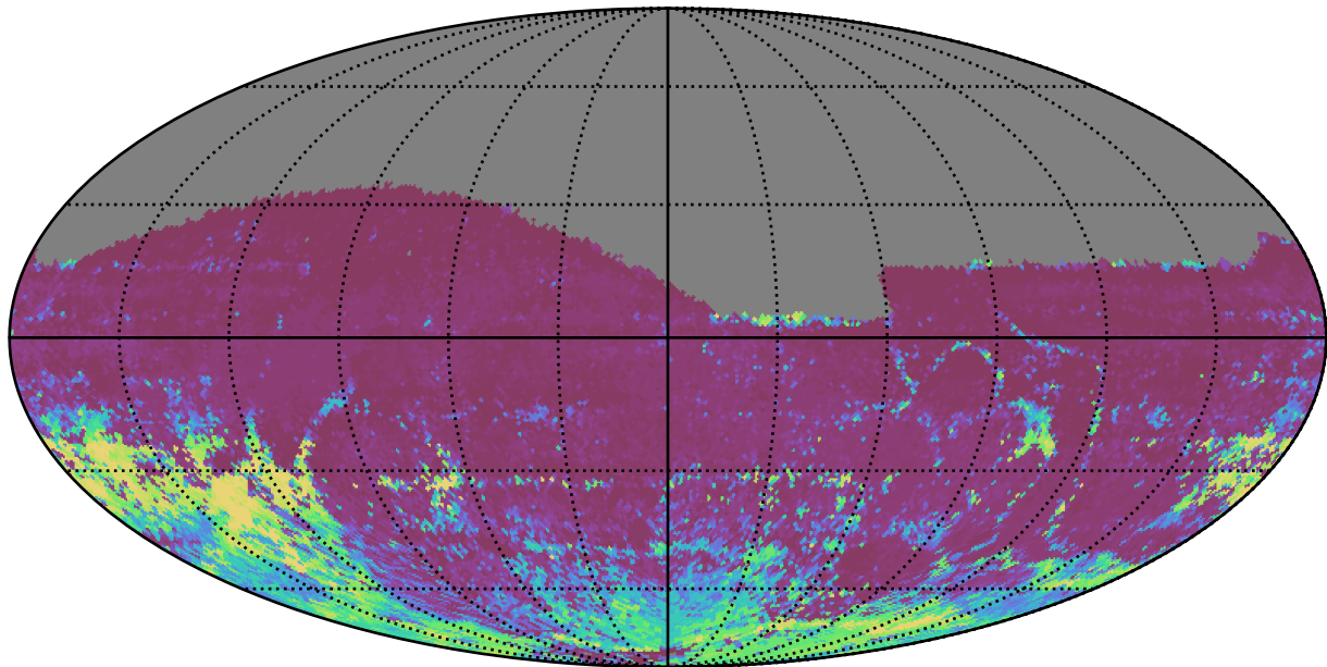
ddf_loaded_half_fl4_v3.4_10yrs All sky r band: 75th Percentile Intranight Timespan
