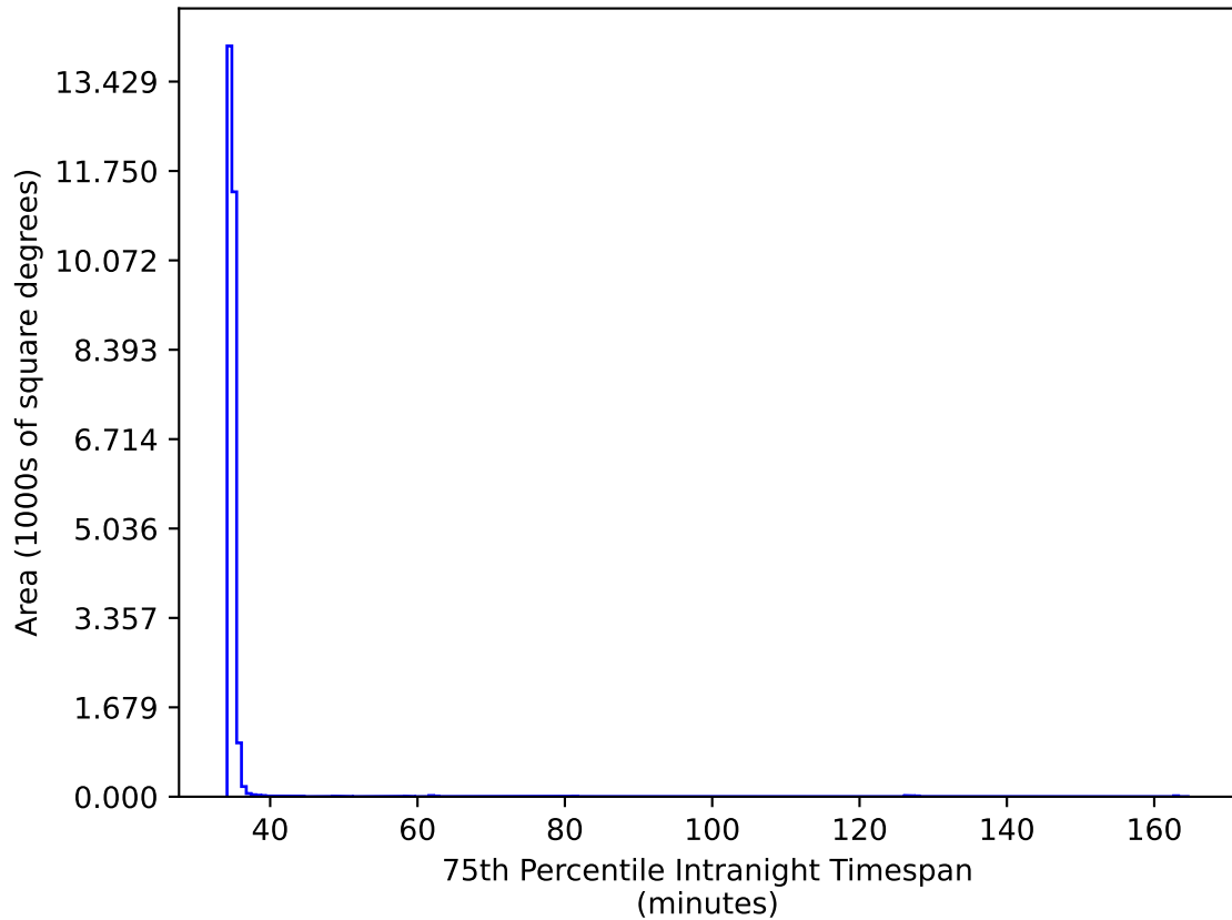
ddf_loaded_half_fl4_v3.4_10yrs All sky iz bands: 75th Percentile Intranight Timespan
