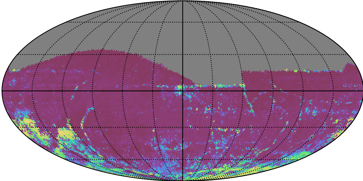
ddf_loaded_half_fl4_v3.4_10yrs All sky i band: 75th Percentile Intranight Timespan
