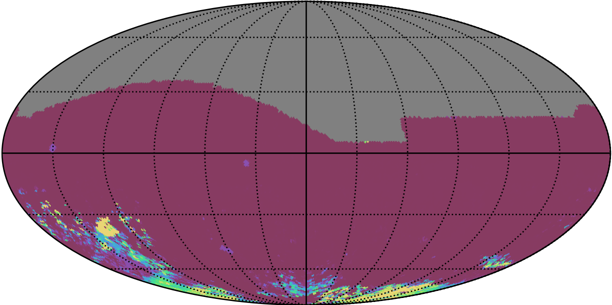
ddf_loaded_half_fl4_v3.4_10yrs All sky gr bands: 75th Percentile Intranight Timespan
