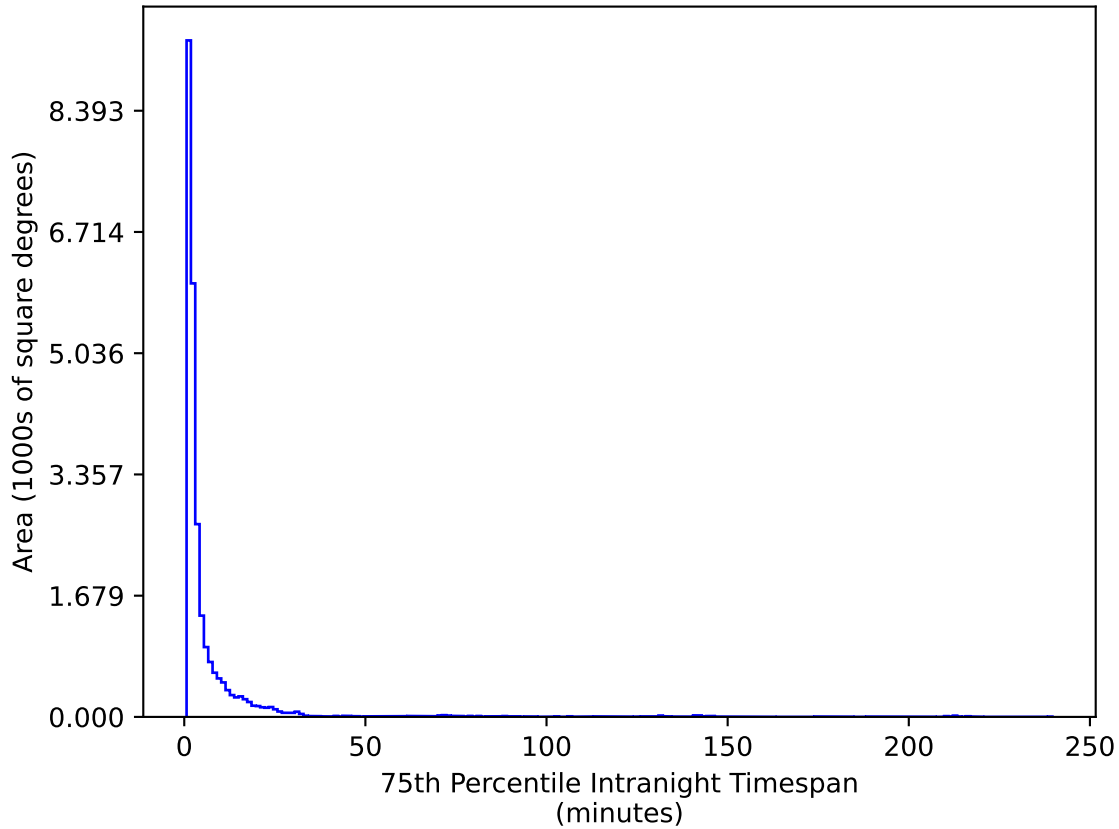
ddf_loaded_half_fl4_v3.4_10yrs All sky g band: 75th Percentile Intranight Timespan
