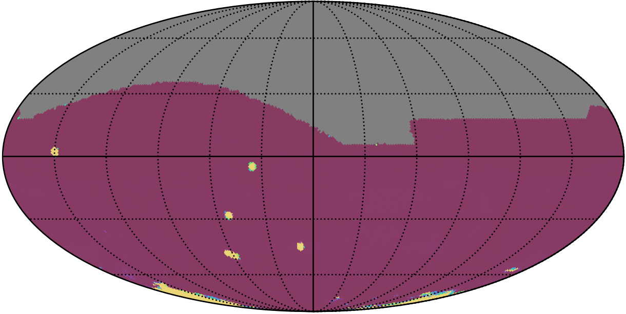
ddf_loaded_half_fl4_v3.4_10yrs All sky all bands: 75th Percentile Intranight Timespan
