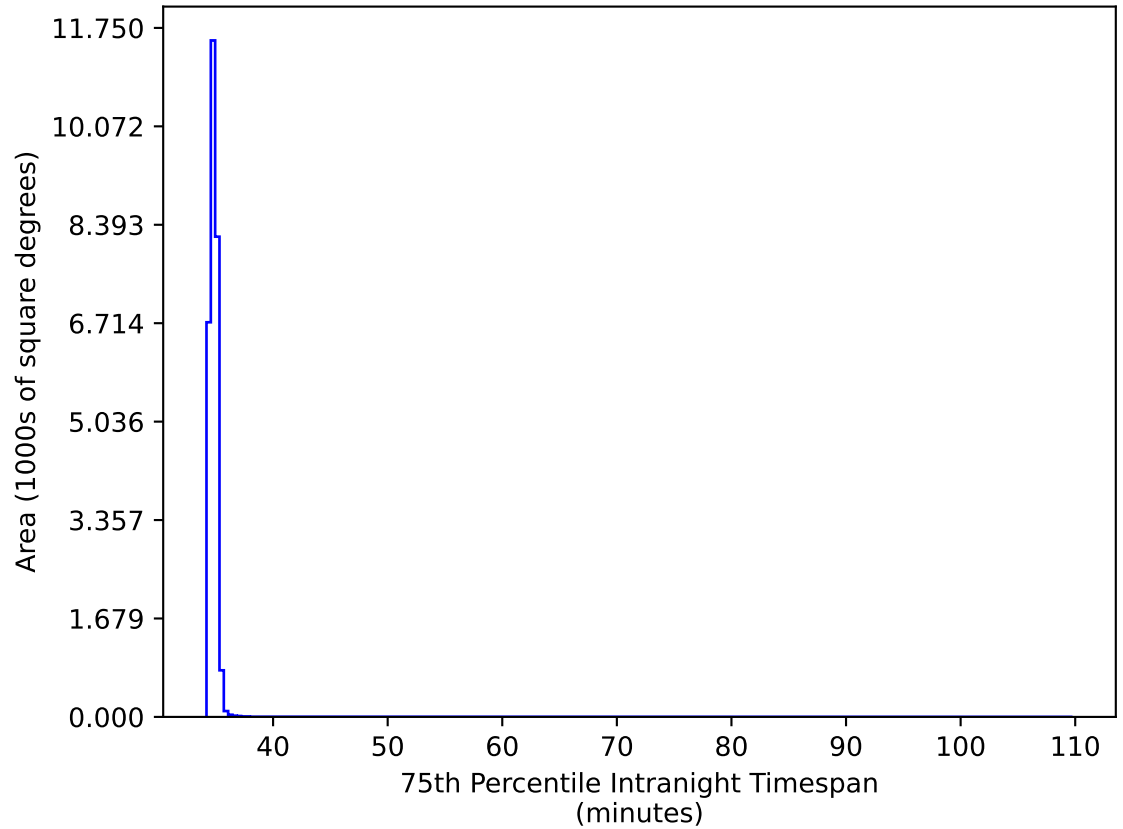
ddf_loaded_half_fl4_v3.4_10yrs All sky all bands: 75th Percentile Intranight Timespan
