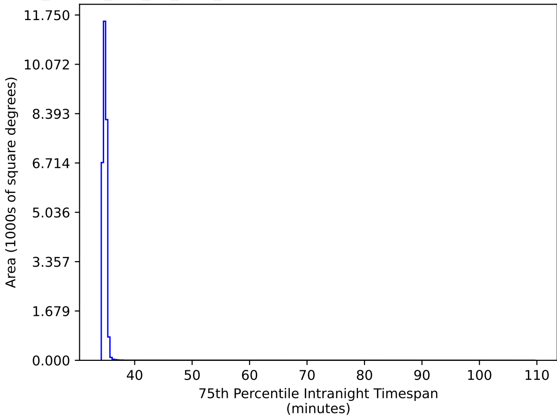
ddf_loaded_half_fl4_v3.4_10yrs All sky: 75th Percentile Intranight Timespan
