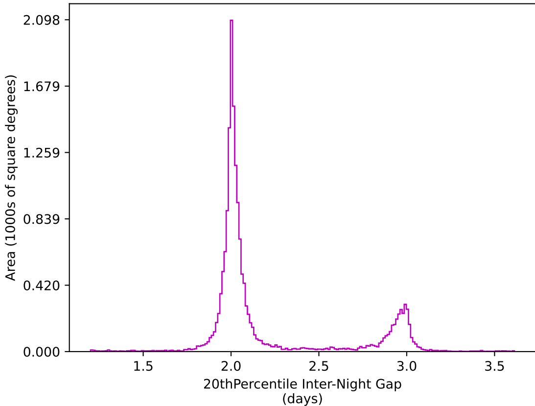
ddf_loaded_half_fl4_v3.4_10yrs WFD z band: 20thPercentile Inter-Night Gap
