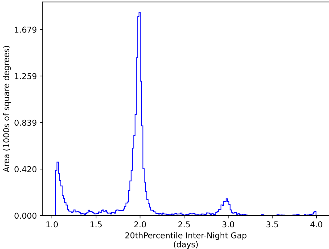
ddf_loaded_half_fl4_v3.4_10yrs WFD y band: 20thPercentile Inter-Night Gap
