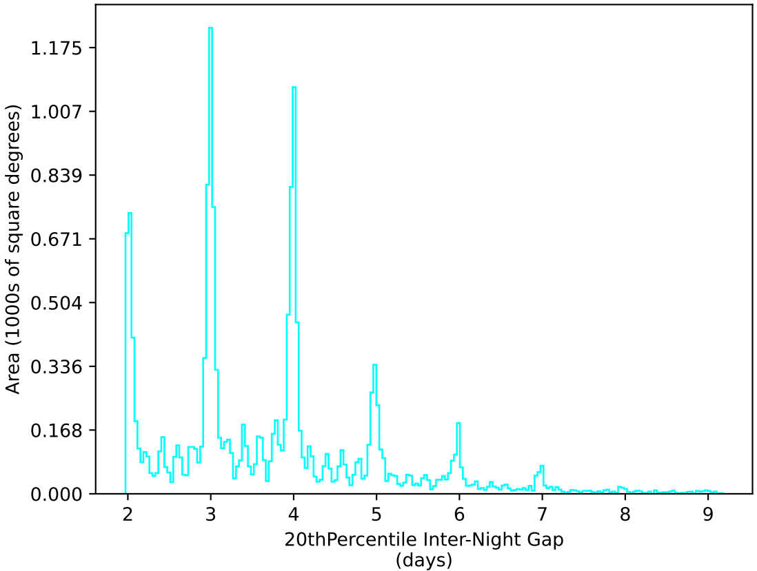
ddf_loaded_half_fl4_v3.4_10yrs WFD u band: 20thPercentile Inter-Night Gap
