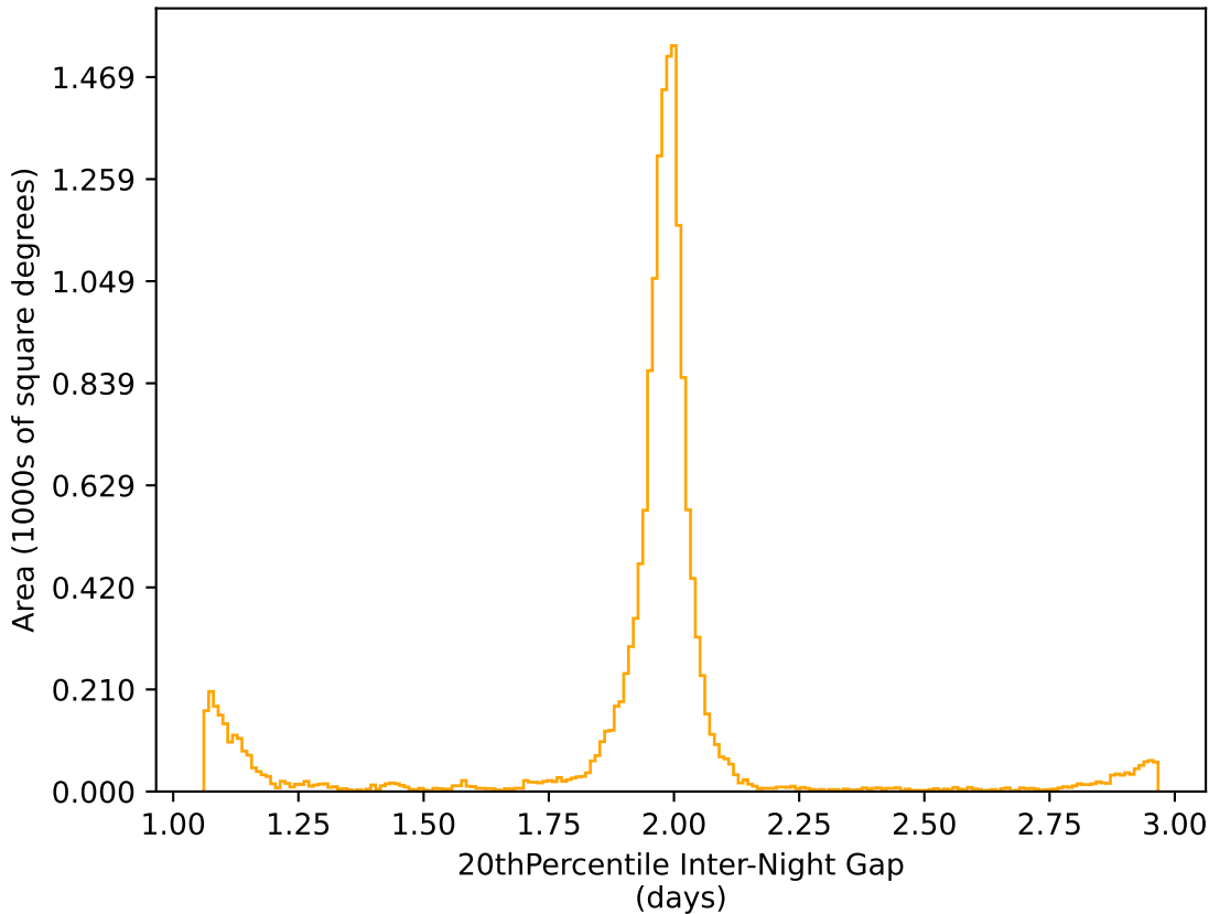
ddf_loaded_half_fl4_v3.4_10yrs WFD r band: 20thPercentile Inter-Night Gap
