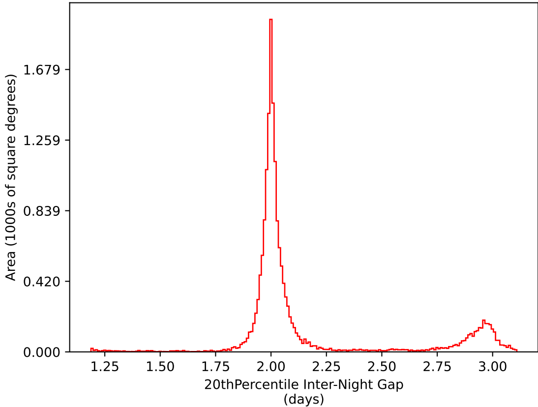
ddf_loaded_half_fl4_v3.4_10yrs WFD i band: 20thPercentile Inter-Night Gap
