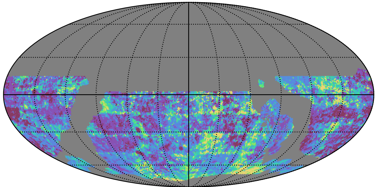
ddf_loaded_half_fl4_v3.4_10yrs WFD g band: 20thPercentile Inter-Night Gap
