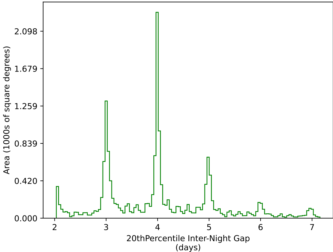
ddf_loaded_half_fl4_v3.4_10yrs WFD g band: 20thPercentile Inter-Night Gap
