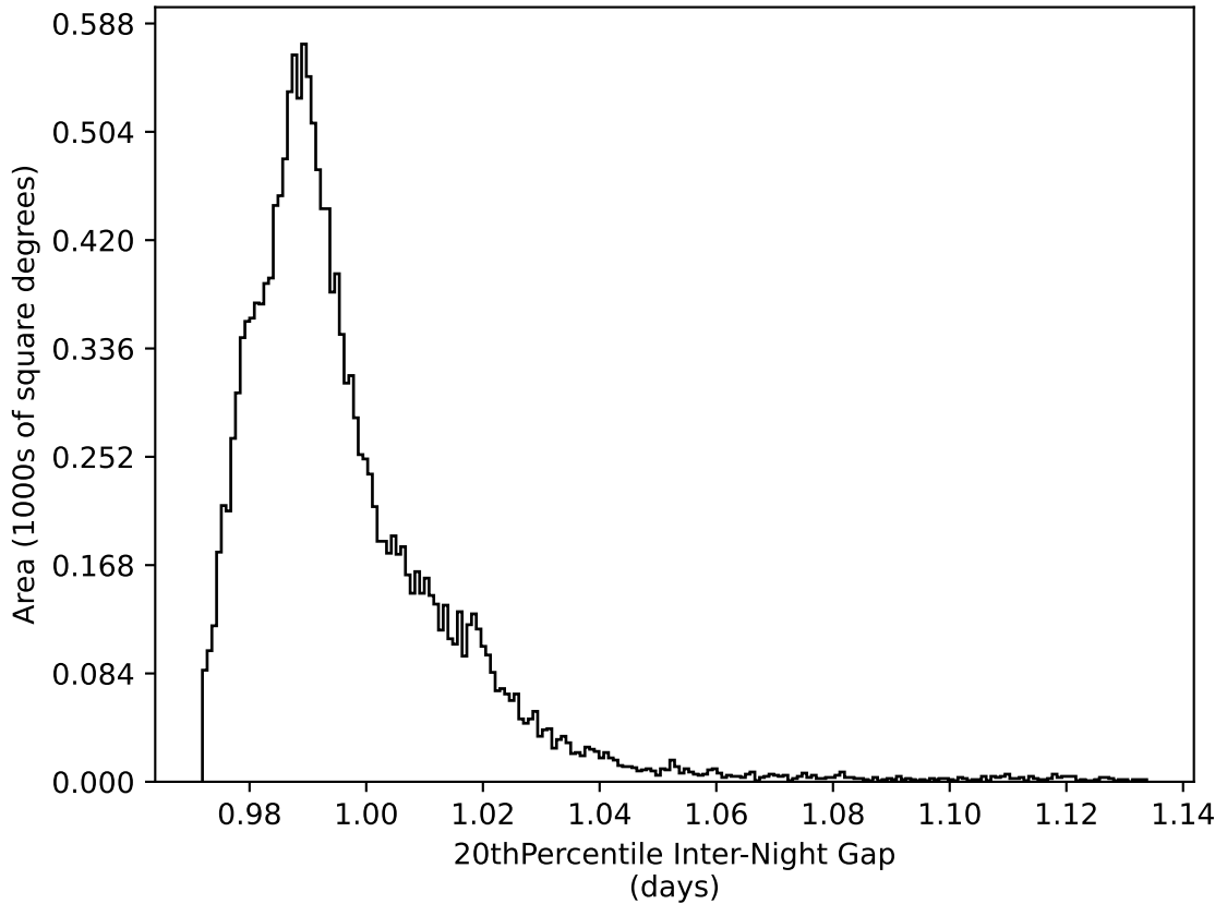
ddf_loaded_half_fl4_v3.4_10yrs WFD all bands: 20thPercentile Inter-Night Gap
