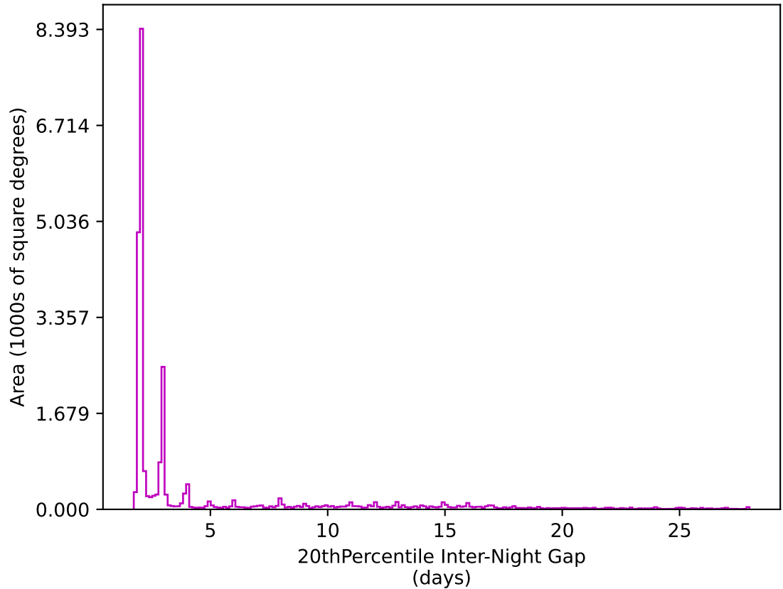
ddf_loaded_half_fl4_v3.4_10yrs All sky z band: 20thPercentile Inter-Night Gap
