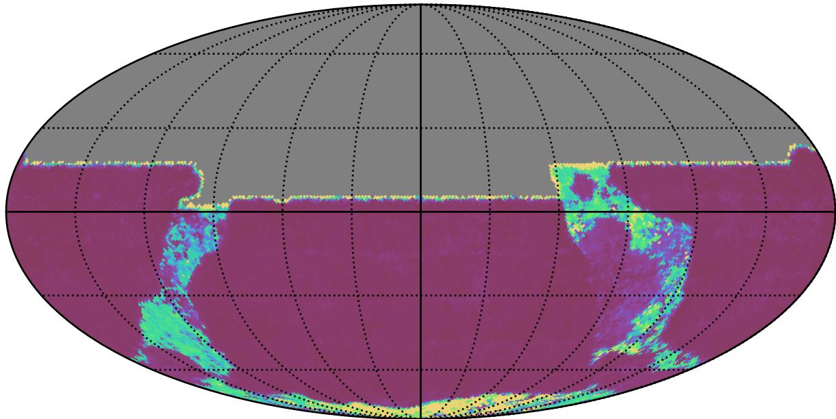
ddf_loaded_half_fl4_v3.4_10yrs All sky y band: 20thPercentile Inter-Night Gap
