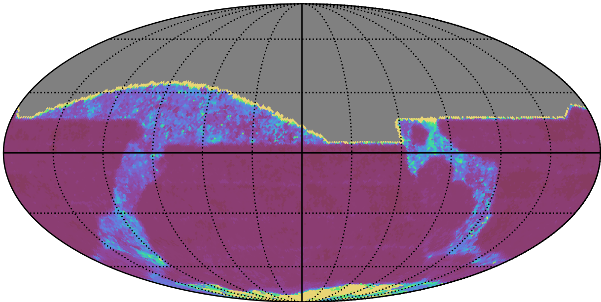
ddf_loaded_half_fl4_v3.4_10yrs All sky r band: 20thPercentile Inter-Night Gap
