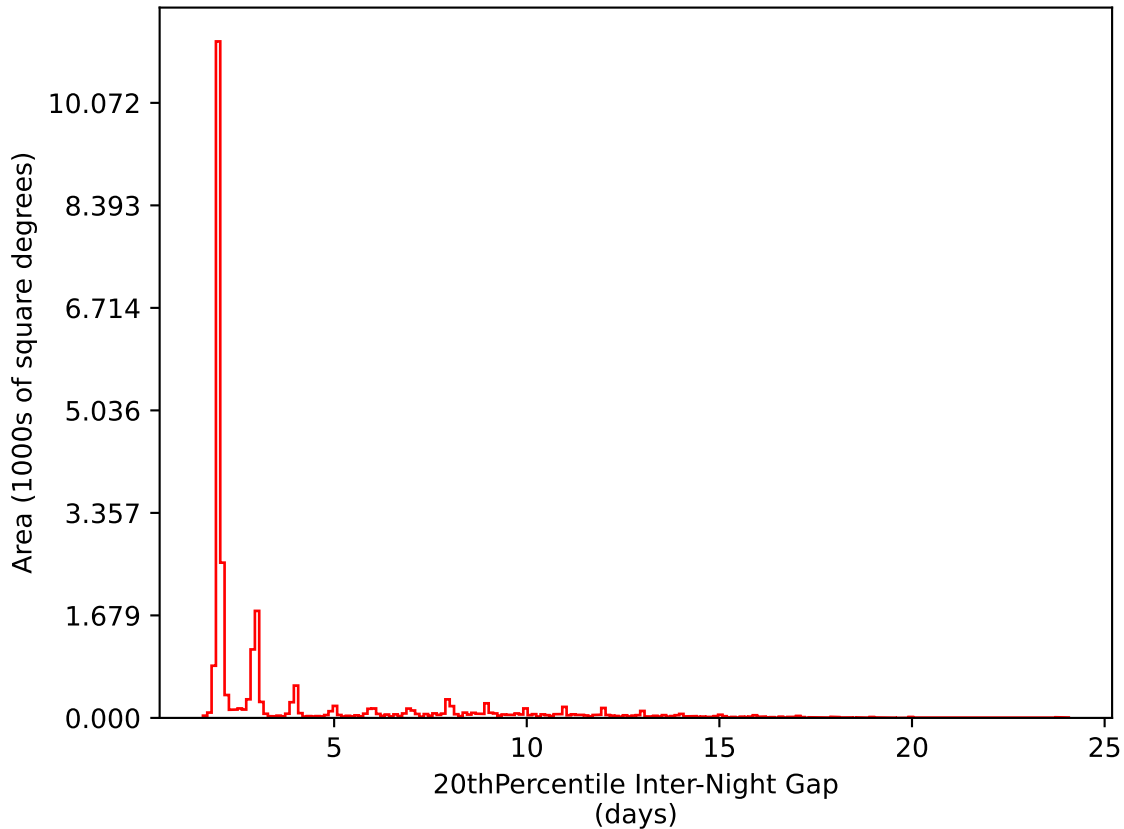
ddf_loaded_half_fl4_v3.4_10yrs All sky i band: 20thPercentile Inter-Night Gap
