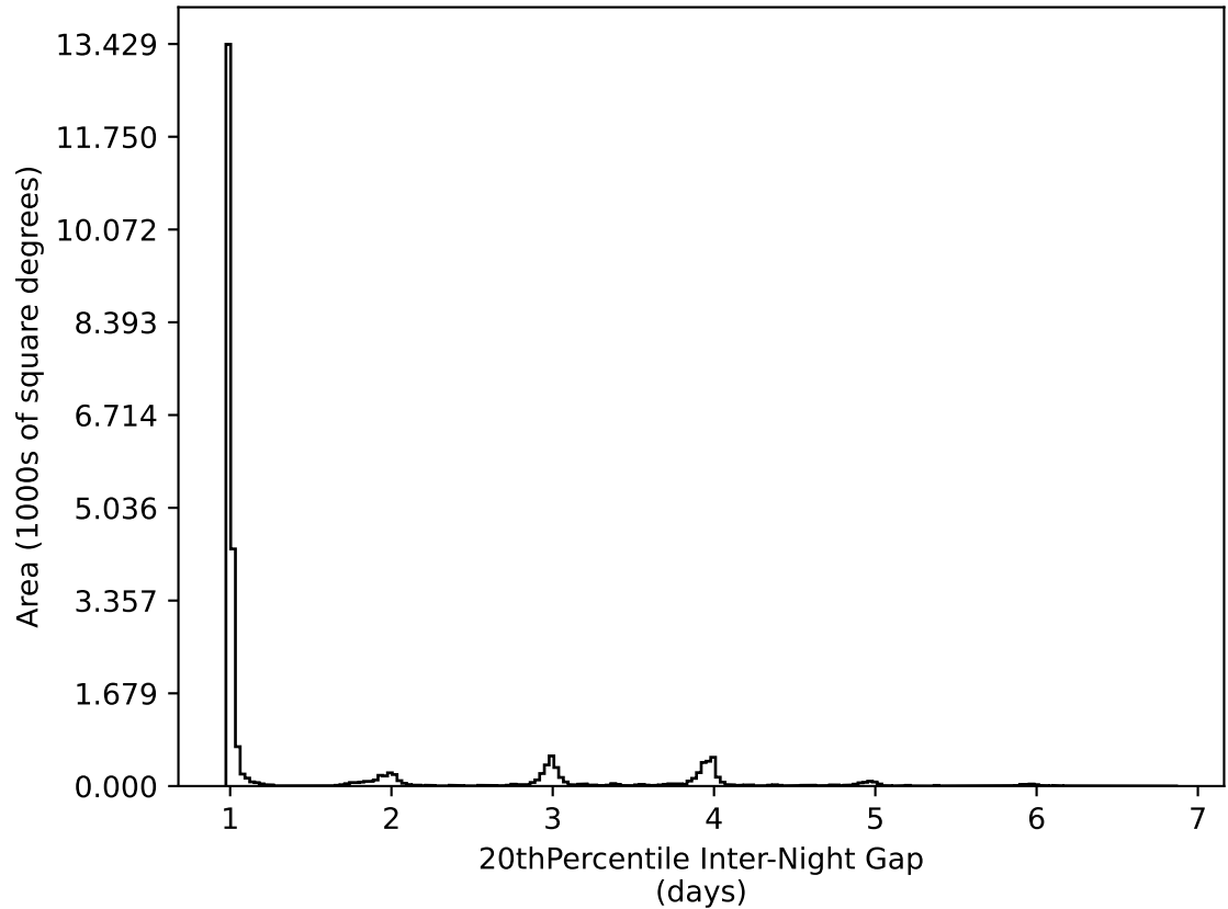
ddf_loaded_half_fl4_v3.4_10yrs All sky all bands: 20thPercentile Inter-Night Gap
