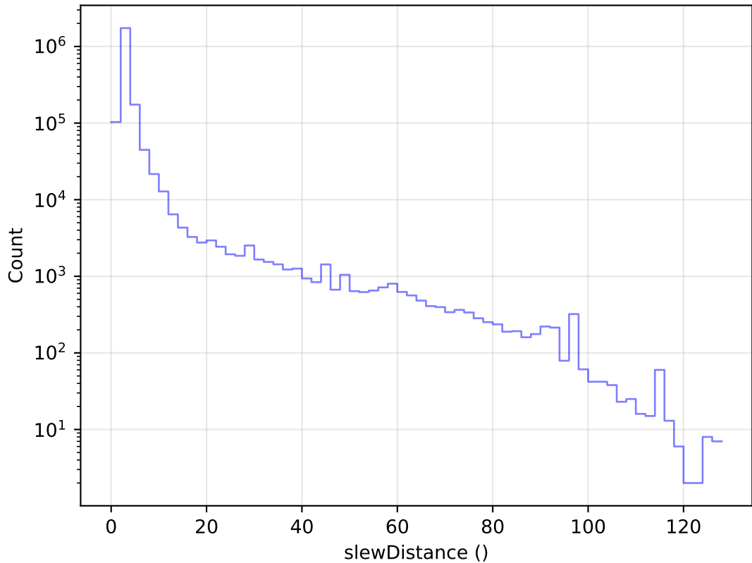
ddf_loaded_half_fl4_v3.4_10yrs All visits: Slew Distance Histogram
