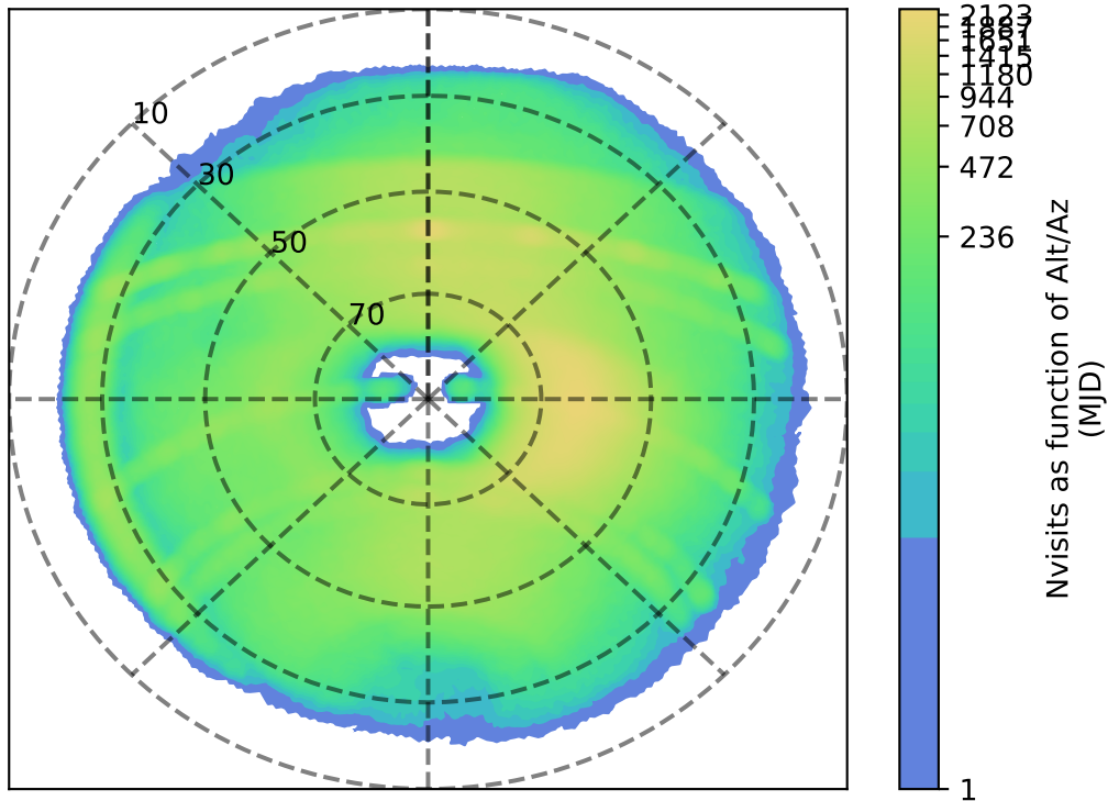
ddf_loaded_half_fl4_v3.4_10yrs r: Nvisits as function of Alt/Az
