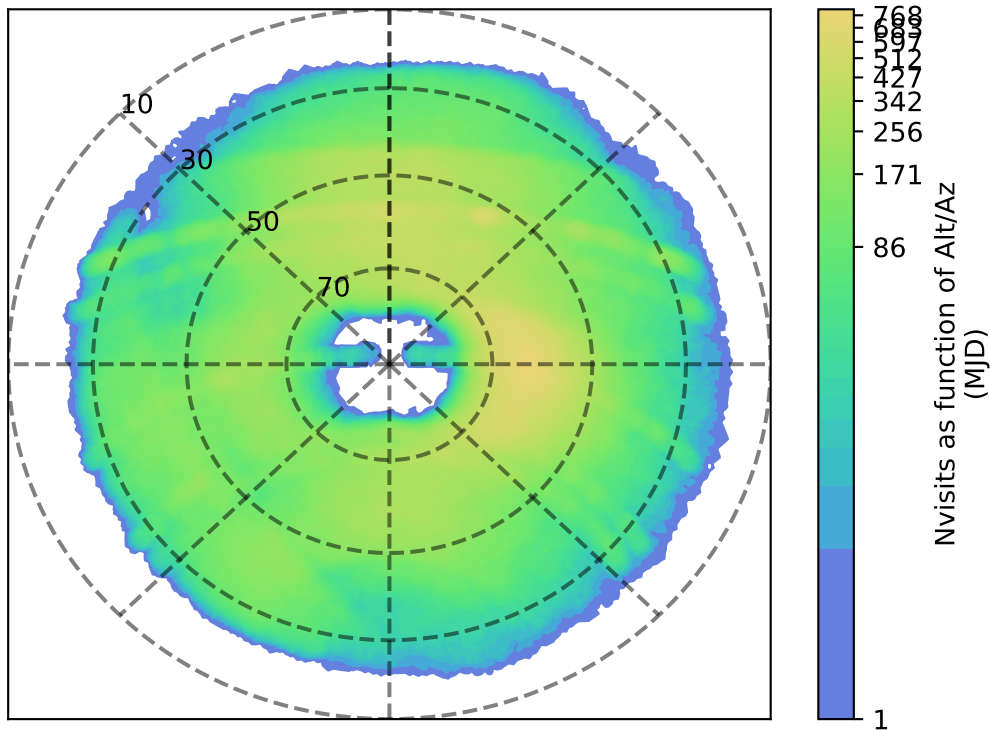
ddf_loaded_half_f14_v3.4_10yrs g: Nvisits as function of Alt/Az
