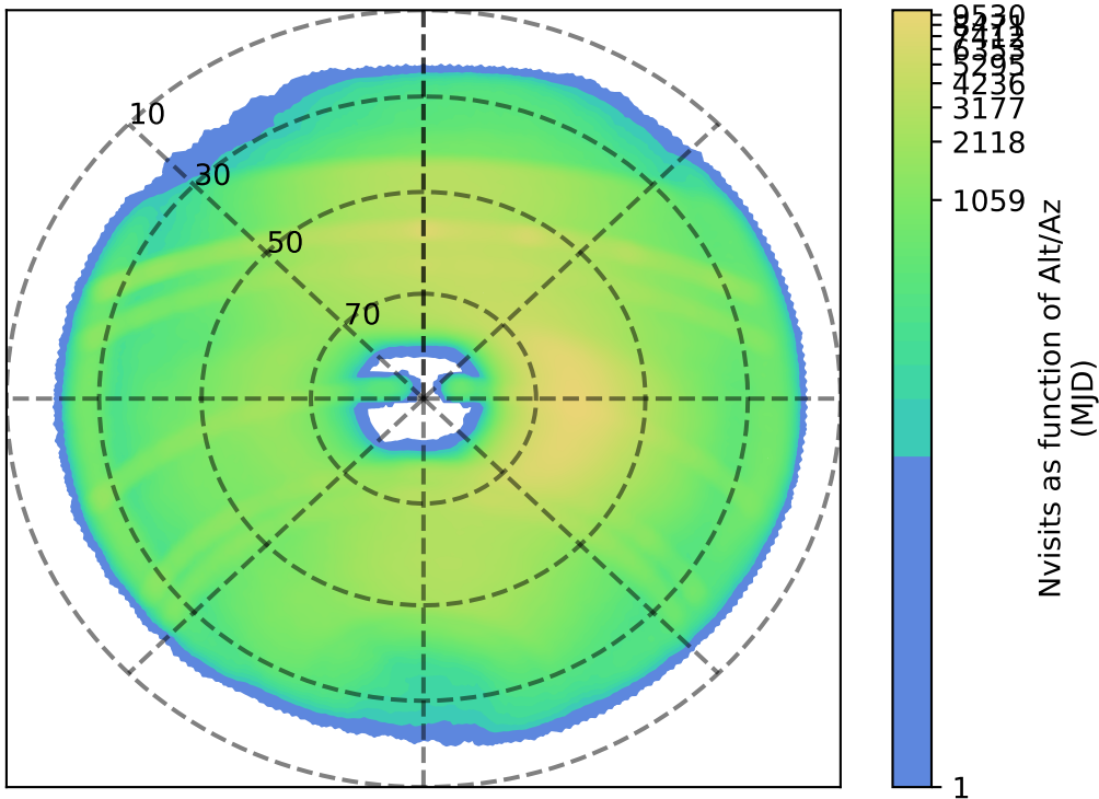
ddf_loaded_half_fl4_v3.4_10yrs : Nvisits as function of Alt/Az
