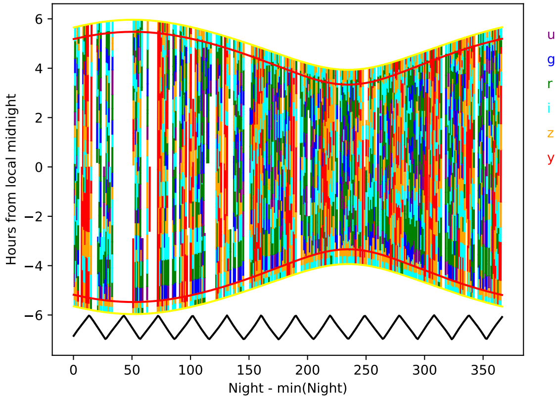
ddf_loaded_half_fl4_v3.4_10yrs year 8-9: Hourglass
