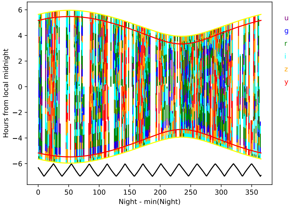
ddf_loaded_half_fl4_v3.4_10yrs year 7-8: Hourglass
