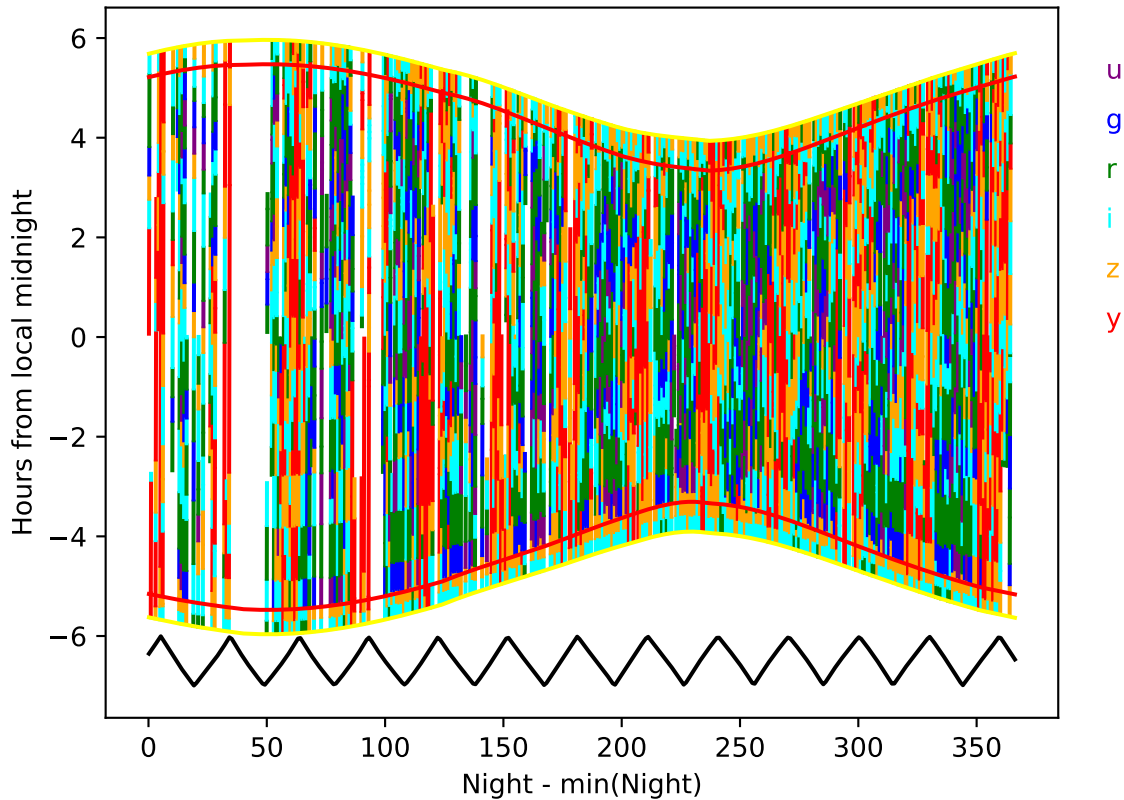
ddf_loaded_half_fl4_v3.4_10yrs year 6-7: Hourglass
