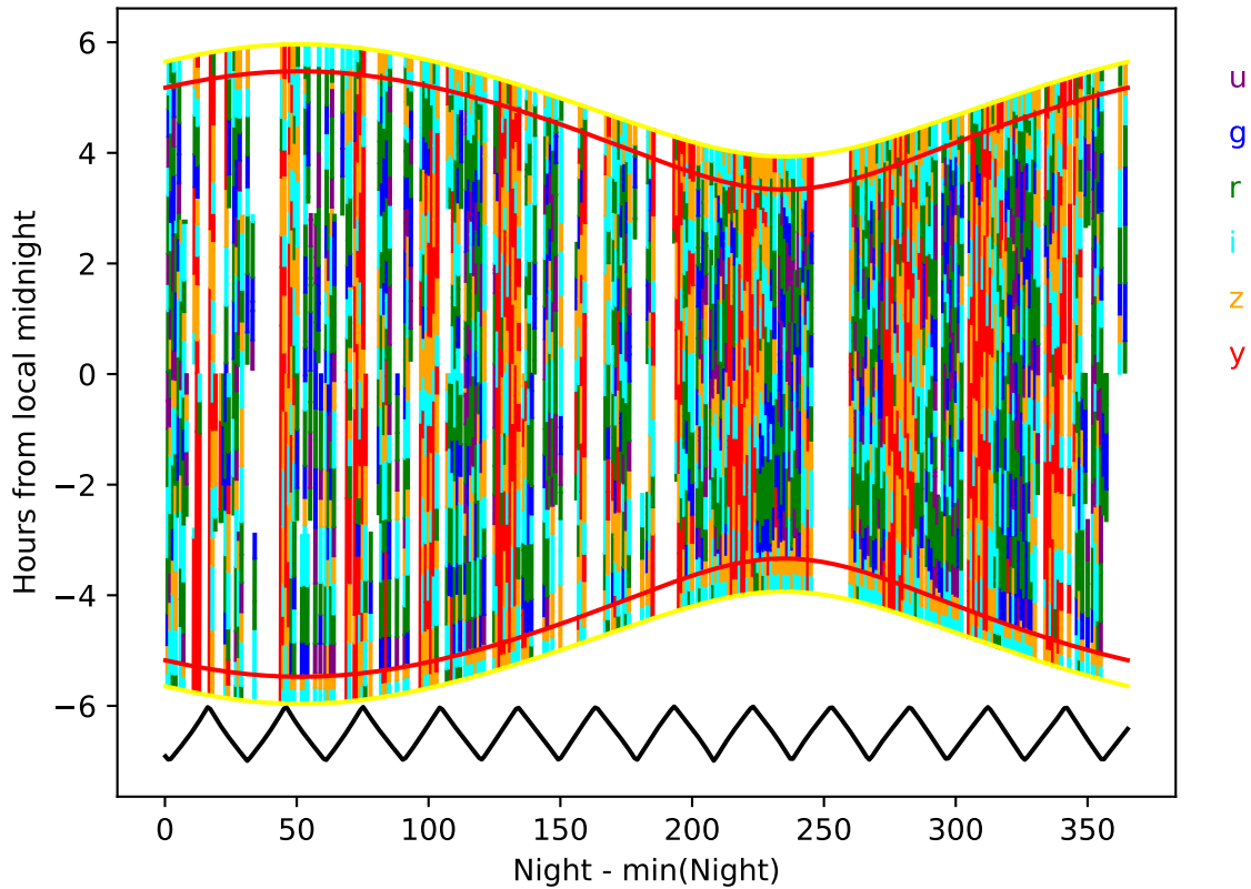
ddf_loaded_half_fl4_v3.4_10yrs year 5-6: Hourglass
