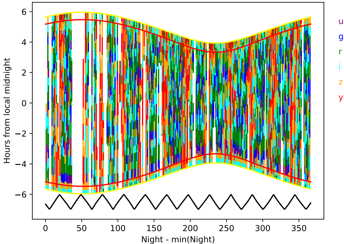
ddf_loaded_half_fl4_v3.4_10yrs year 2-3: Hourglass
