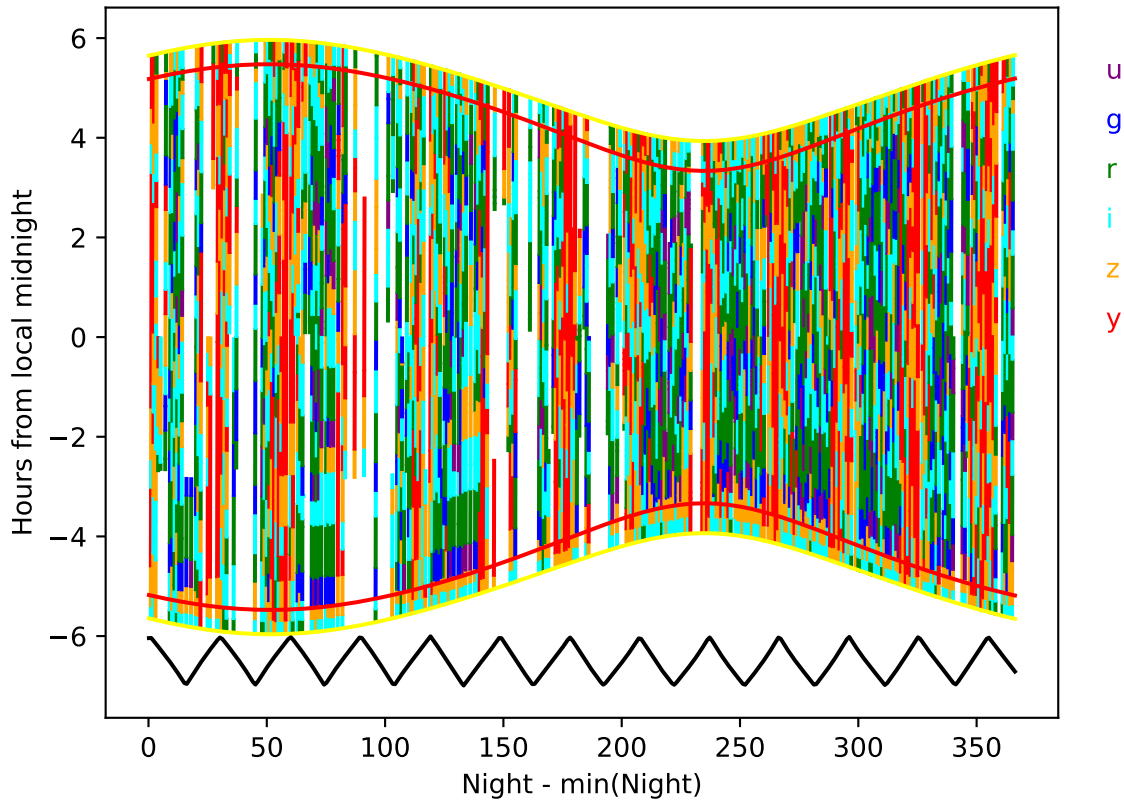
ddf_loaded_half_fl4_v3.4_10yrs year 1-2: Hourglass
