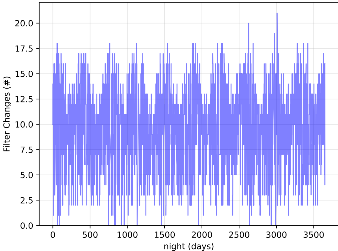
ddf_loaded_half_fl4_v3.4_10yrs : Filter Changes
