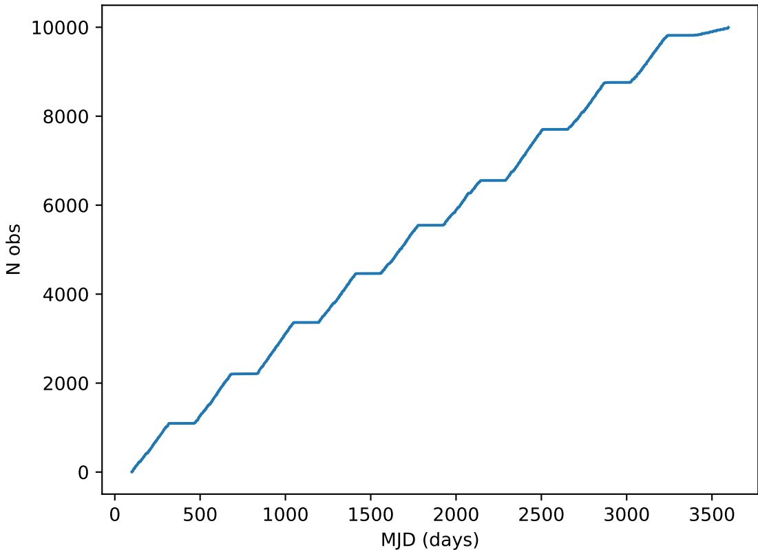
ddf_loaded_half_fl4_v3.4_10yrs note like DD:EDFS_b%: Cumulative
