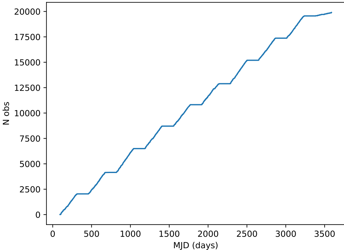
ddf_loaded_half_fl4_v3.4_10yrs note like DD:ECDFS%: Cumulative
