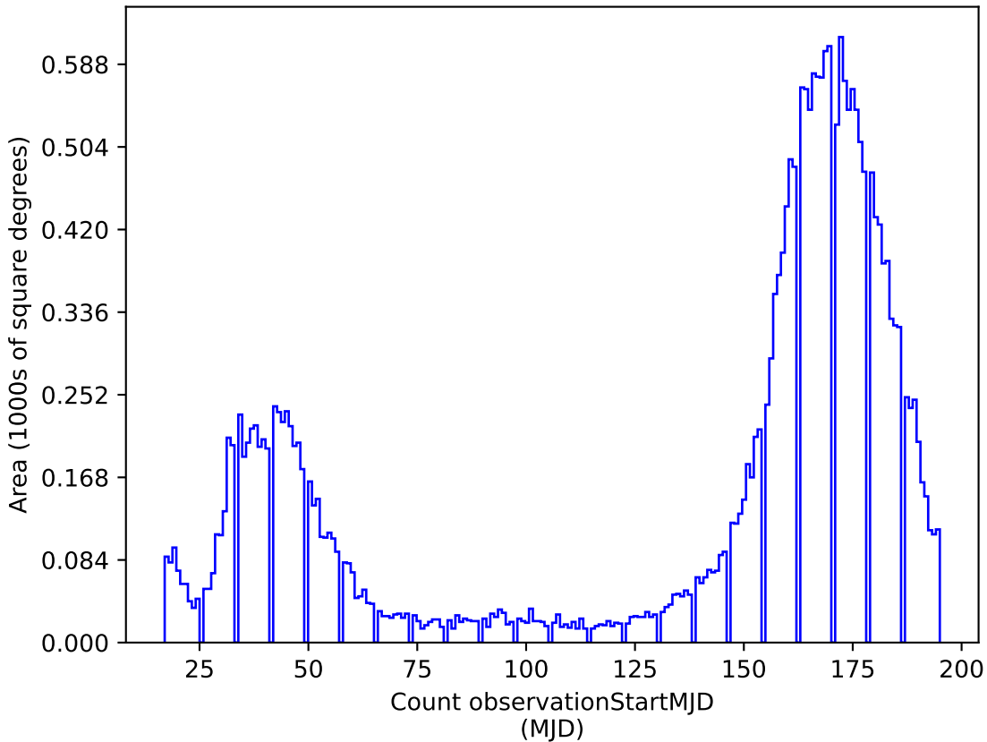
ddf_loaded_half_fl4_v3.4_10yrs z: Count observationStartMJD
