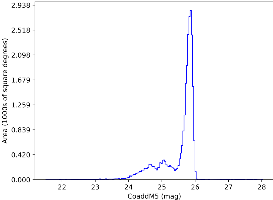
ddf_loaded_half_f14_v3.4_10yrs z: CoaddM5
