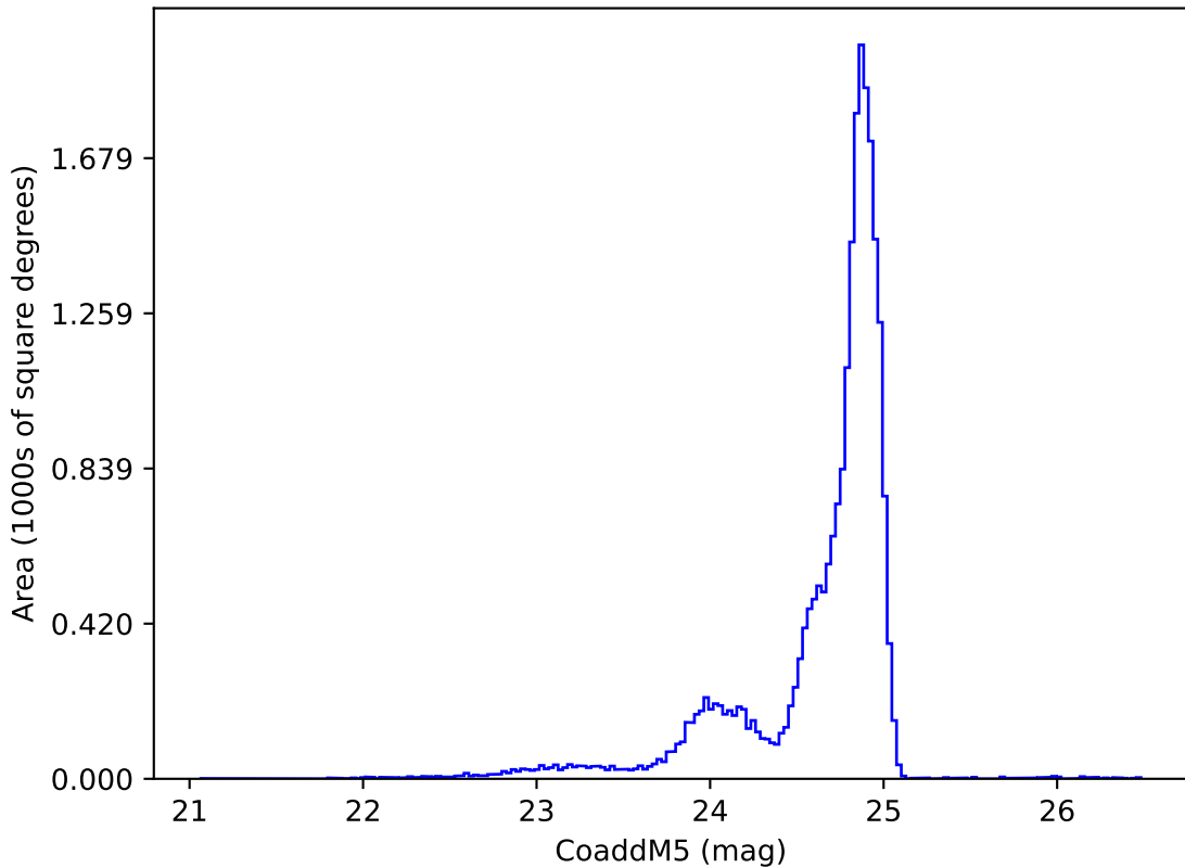
ddf_loaded_half_f14_v3.4_10yrs y: CoaddM5
