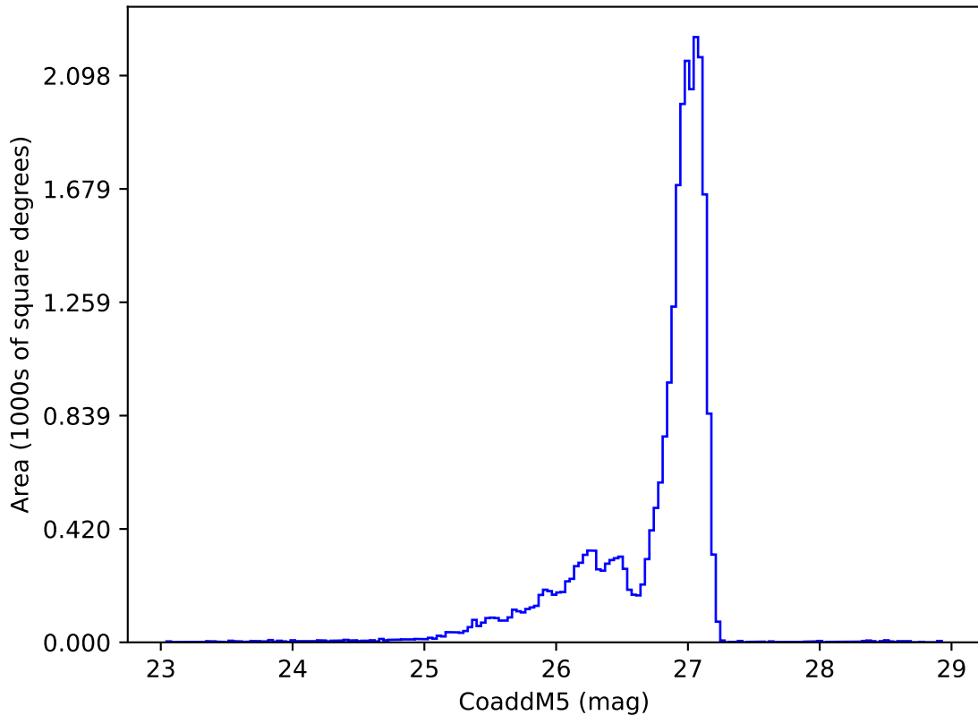
ddf_loaded_half_f14_v3.4_10yrs r: CoaddM5
