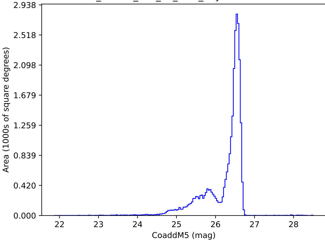
ddf_loaded_half_fl4_v3.4_10yrs i: CoaddM5
