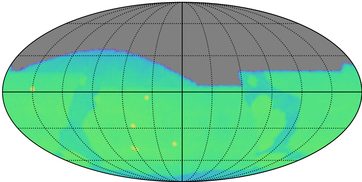
ddf_loaded_half_fl4_v3.4_10yrs g: CoaddM5
