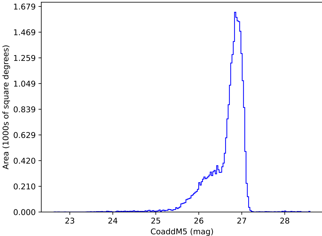
ddf_loaded_half_fl4_v3.4_10yrs g: CoaddM5
