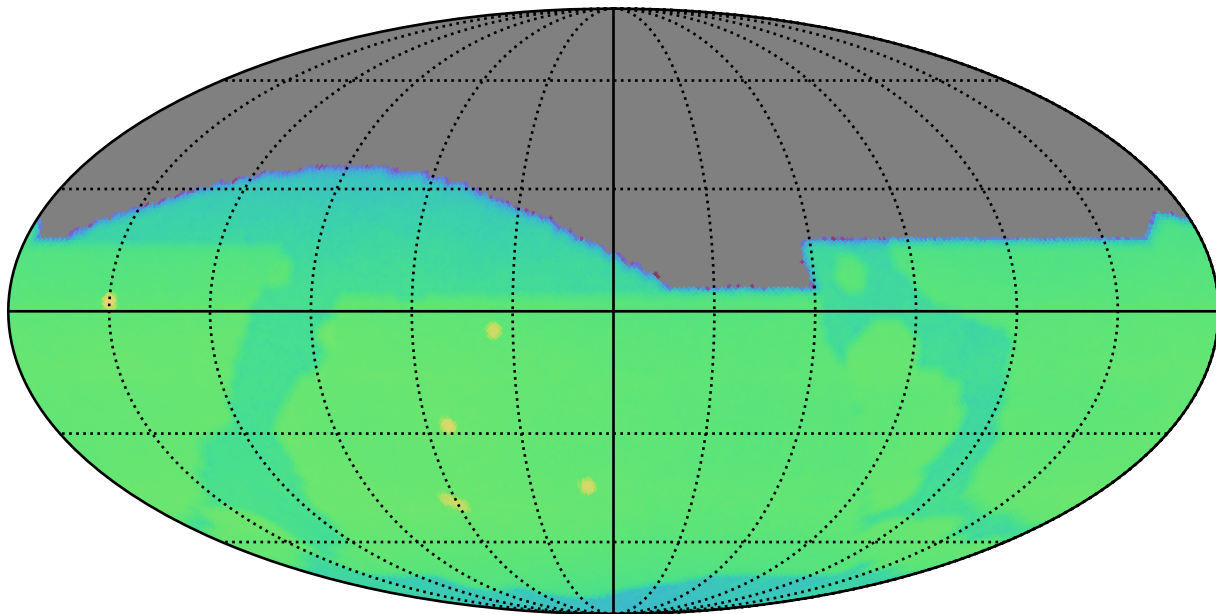
ddf_loaded_half_fl4_v3.4_10yrs : CoaddM5
