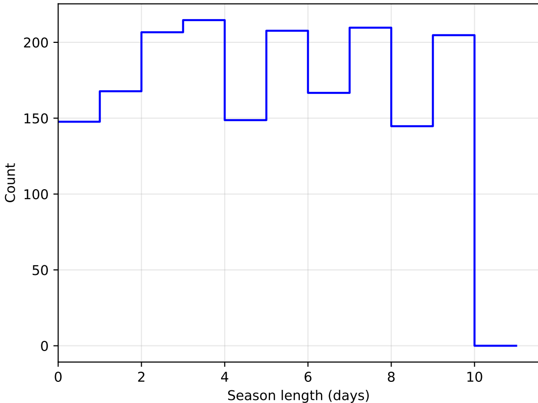
ddf_loaded_half_fl4_v3.4_10yrs DD:WFD all bands: SeasonLength
