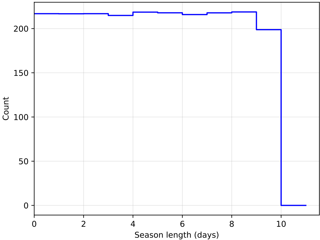
ddf_loaded_half_fl4_v3.4_10yrs DD:EDFS all bands: SeasonLength
