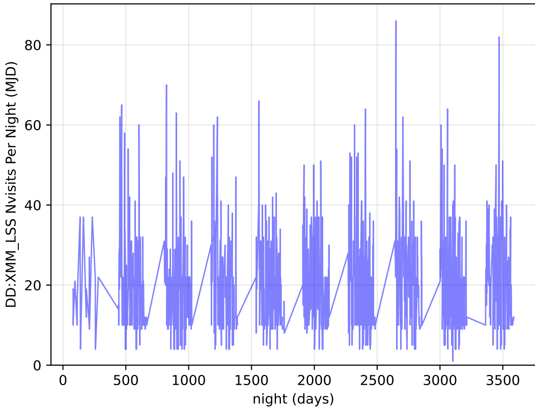
ddf_loaded_half_fl4_v3.4_10yrs all bands: DD:XMM_LSS Nvisits Per Night
