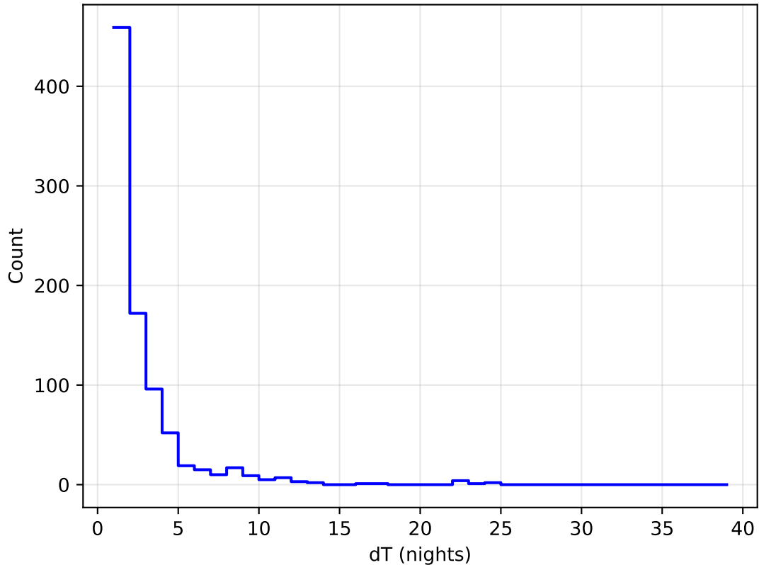
ddf_loaded_half_fl4_v3.4_10yrs all bands: DD:XMM_LSS Delta Nights Histogram
