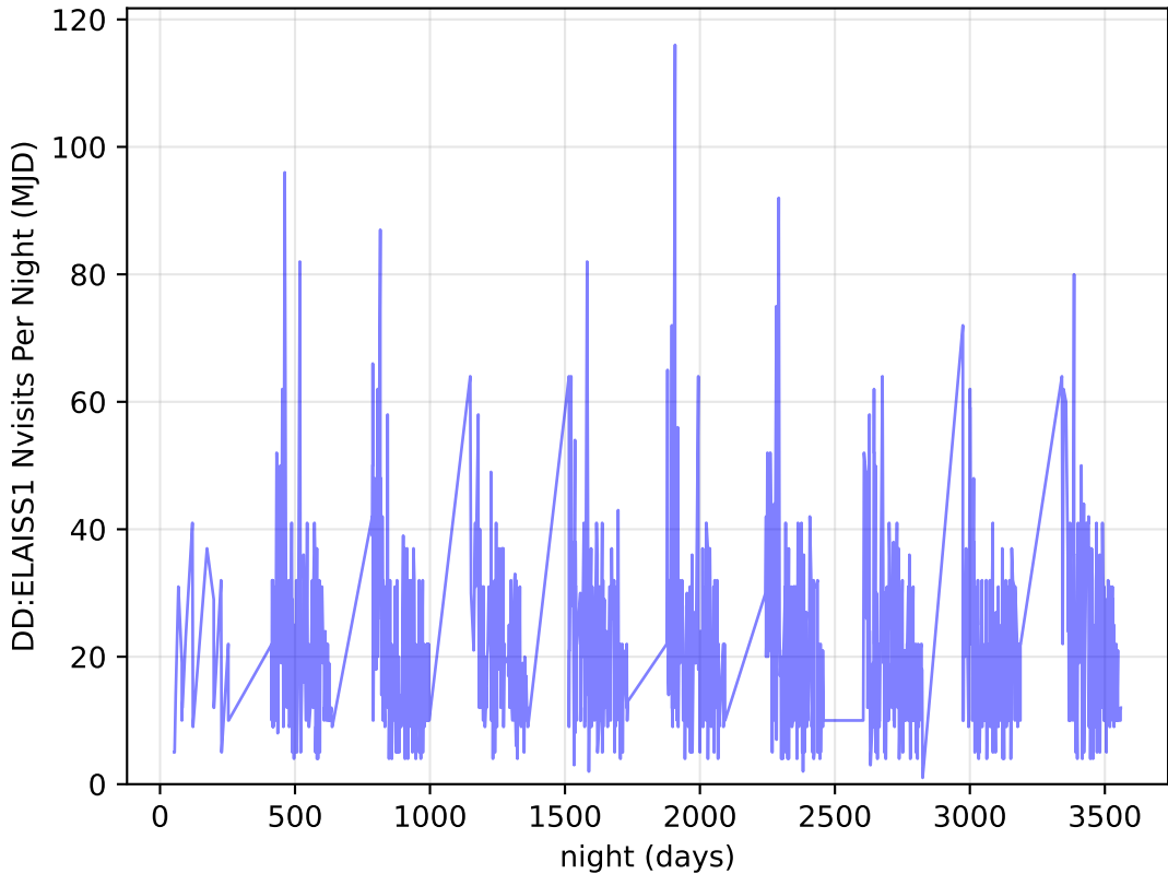
ddf_loaded_half_fl4_v3.4_10yrs all bands: DD:ELAISS1 Nvisits Per Night
