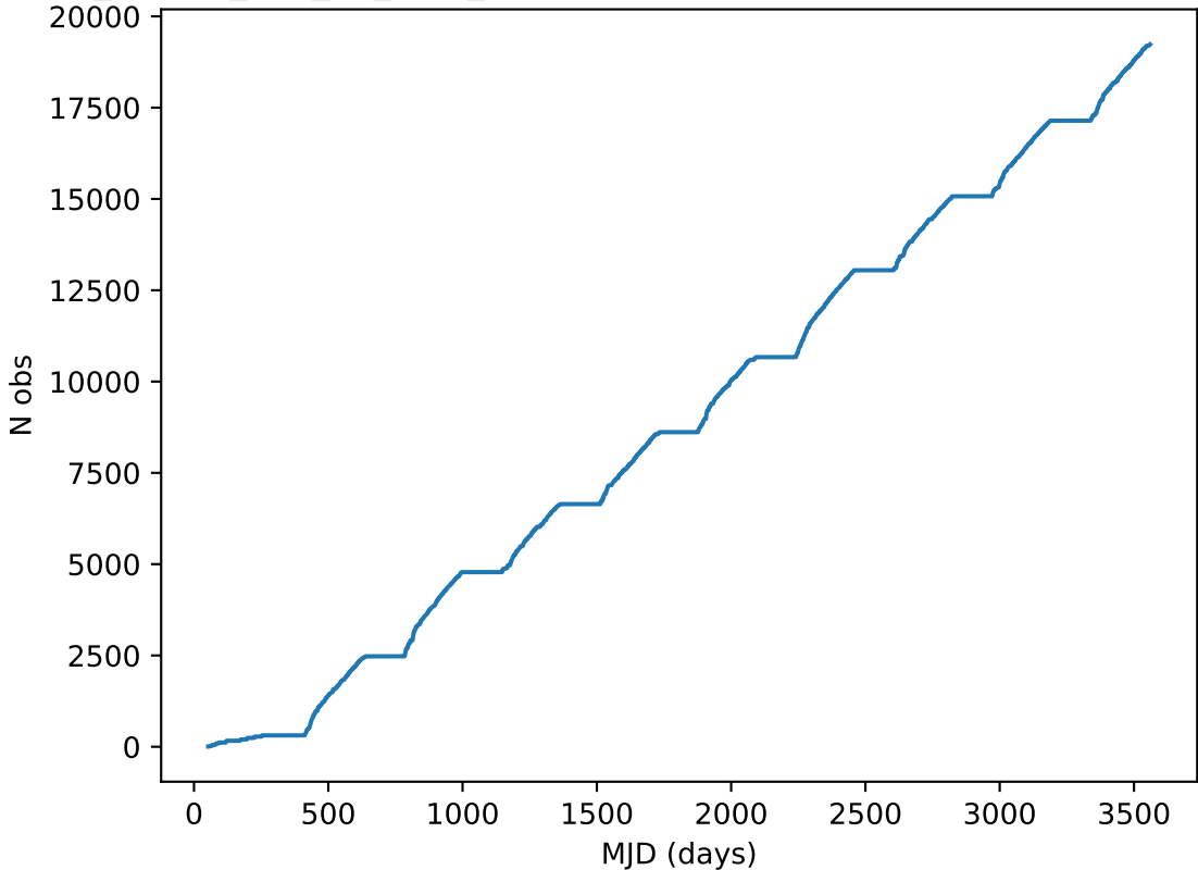
ddf_loaded_half_fl4_v3.4_10yrs all bands: DD:ELAISS1 Cumulative NVisits
